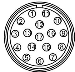
Socket Face
