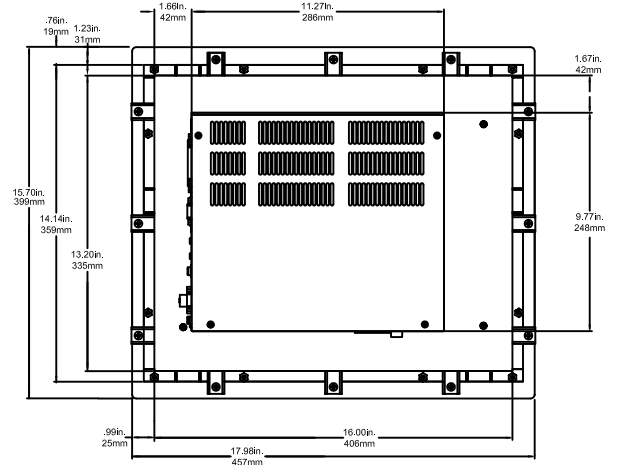
HPC HPX 17" Back View
