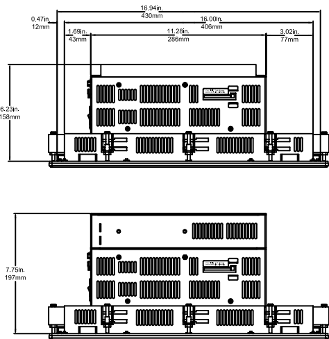
HPC HPX 17" Bottom View Base and PCI Expansion
