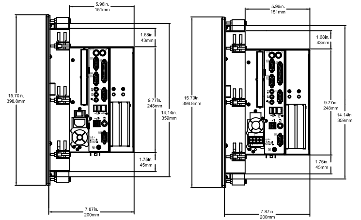
HPC HPX 17" Right View with 3/4 Length PCI Expansion
