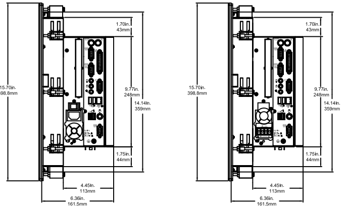
HPC HPX 17" Right View AC and DC
