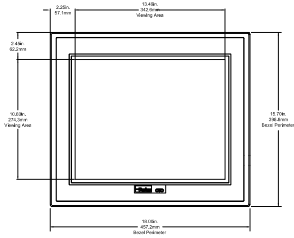
HPC HPX 17" Front View
